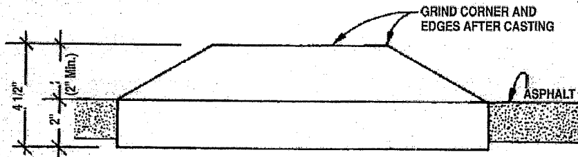
Figure 2: Speed Breaker Detail
