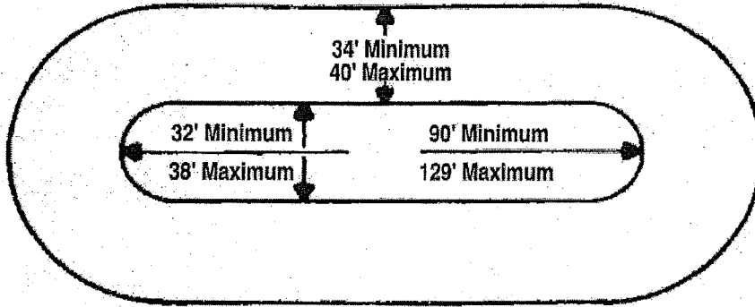
Figure 1: Track Dimension Detail
